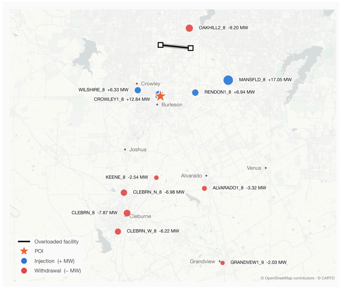
Figure: 100 MW illustrated-contingency dispatch, showing injecting and withdrawing nodes relative to Burleson Switch and the overloaded facility.
