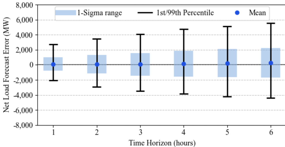
Figure 5: Net Load Forecast Error Across Different Time Horizon Durations
