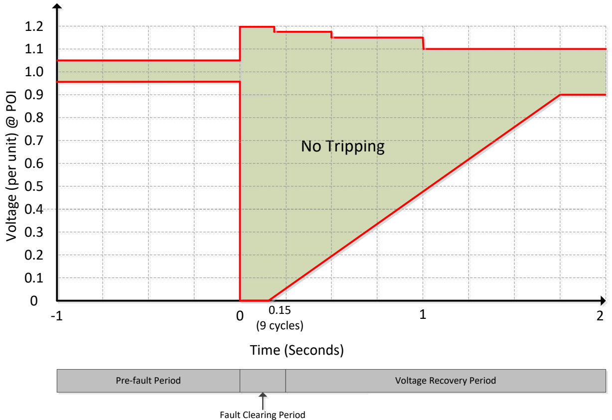
Figure 1: Default Voltage Ride-Through Boundaries for IRRs Connected to the ERCOT Transmission Grid
