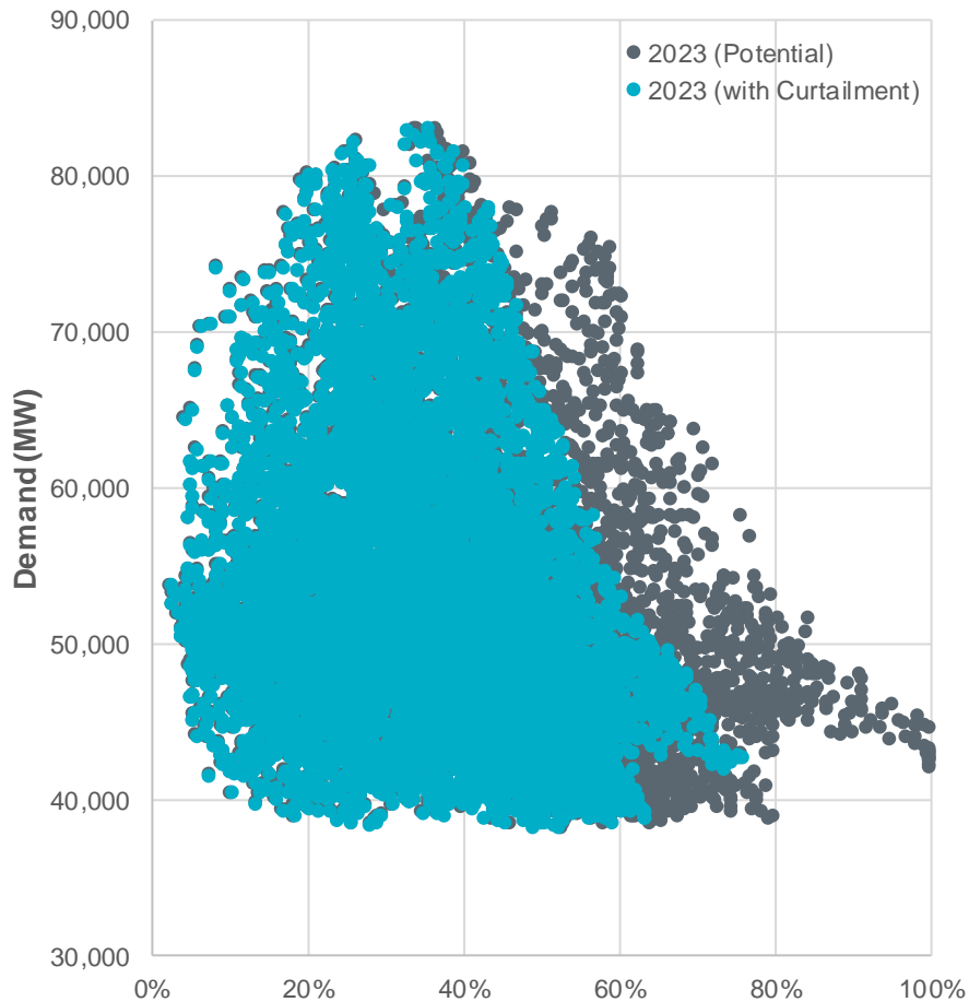
2023 Solar and Wind Penetration
