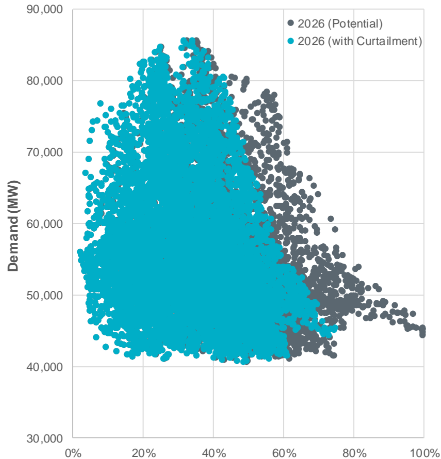
2026 Solar and Wind Penetration
