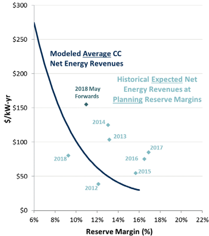
Figure 4 Average Modeled vs. Historical Expected Net Energy Revenues by Reserve Margin
