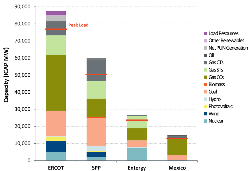
Figure A1-9 Resource Mix for ERCOT and Neighboring System
