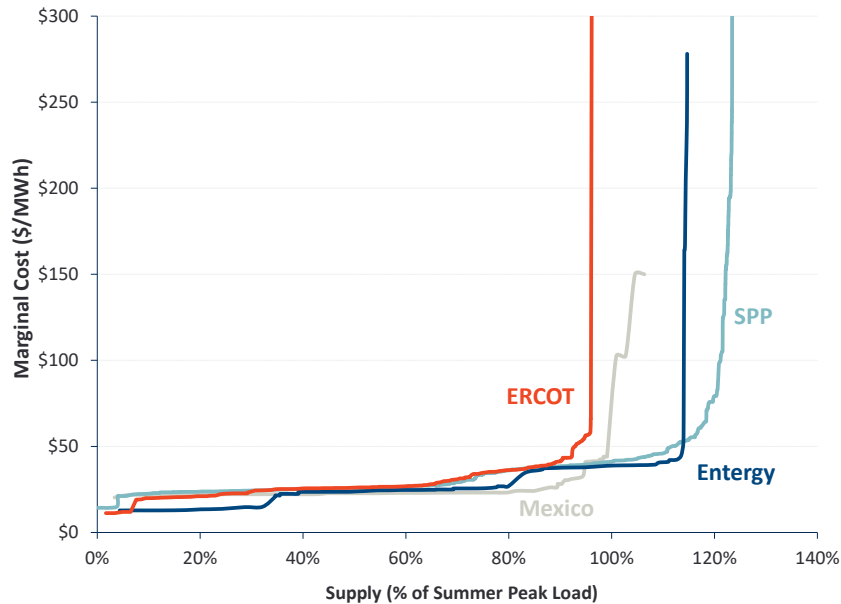
Figure A1-10 2022 System Supply Curves
