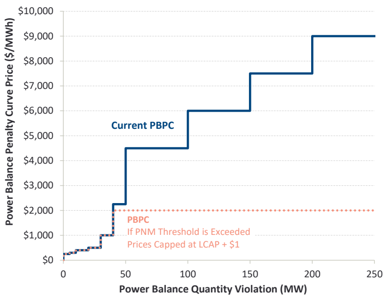
Figure A1-12 Power Balance Penalty Curve
