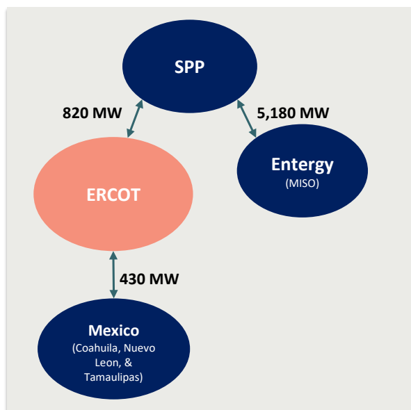
Figure A1-8 System Topology and Modeled Inerties
