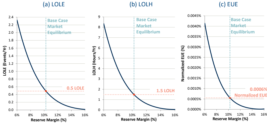
Figure 10 Reliability Metrics that Vary with Reserve Margins
