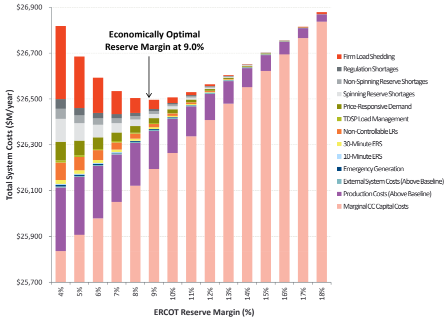
Figure 8 Total System Costs across Planning Reserve Margins
