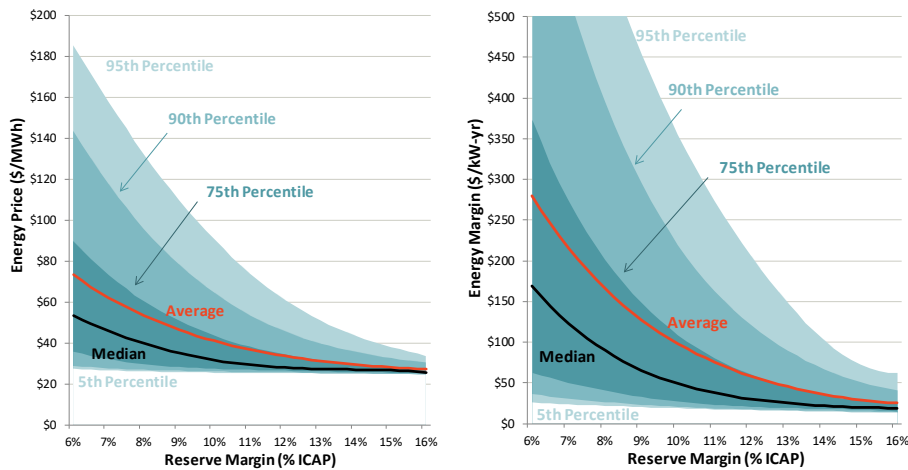
Distribution of Spot Energy Prices (Left) and Net Energy Revenues for a Marginal Unit (Right)
