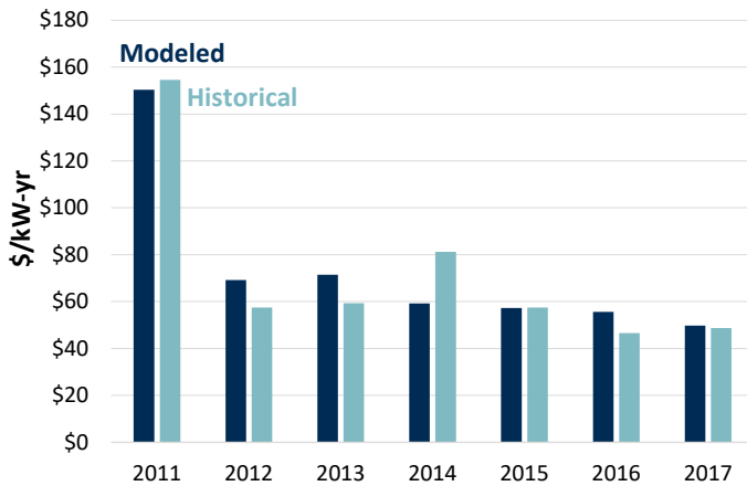
Figure 3 Modeled vs. Actual Combined-Cycle Net Energy Revenues
