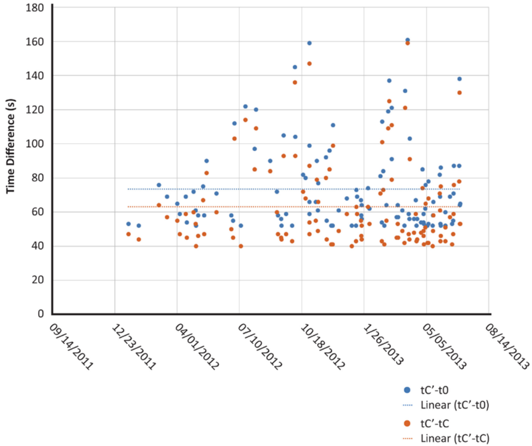
Figure A.30: Eastern Interconnection t_{C'}-t_0 (blue) and t_{C'}-t_C (orange) time-based measures
