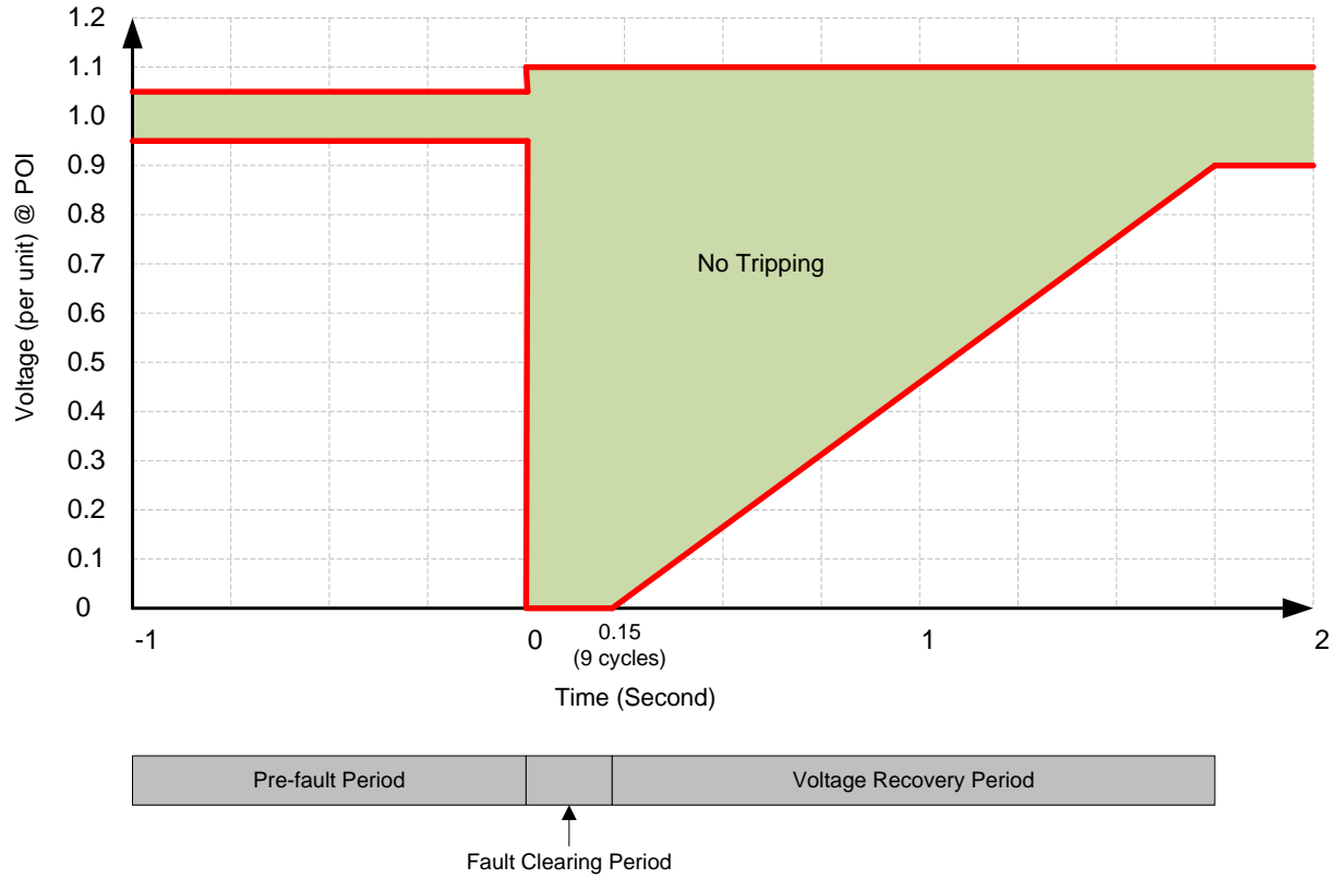
Figure 1: Default Voltage Ride-Through Boundaries For IRRs. The default clearing period is nine cycles or 0.15 seconds. Recovery time to +/-10% of per unit voltage should be within 105 cycles, or 1.75 seconds. IRRs should not trip for system voltages within the boundary.
