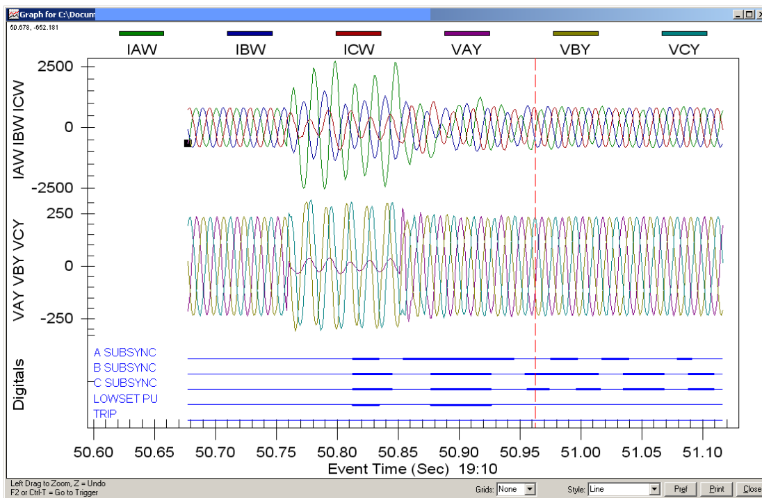
Figure 11: Algorithm Response to an EHV Single Phase Bus Fault
