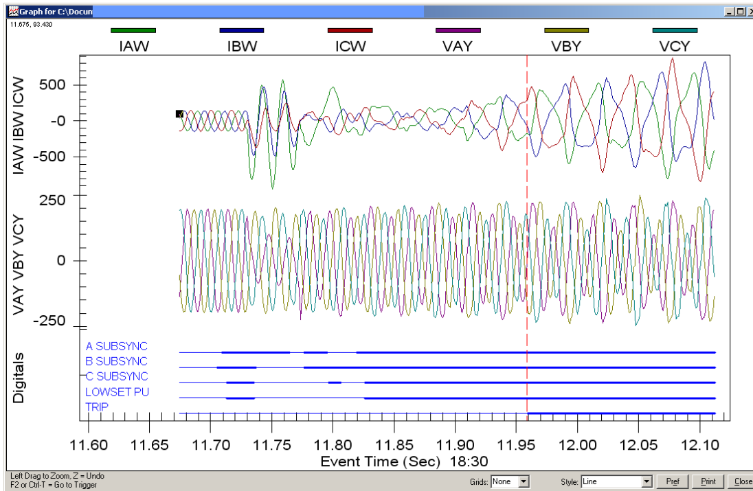
Figure 10: Algorithm Response to the Actual Event
