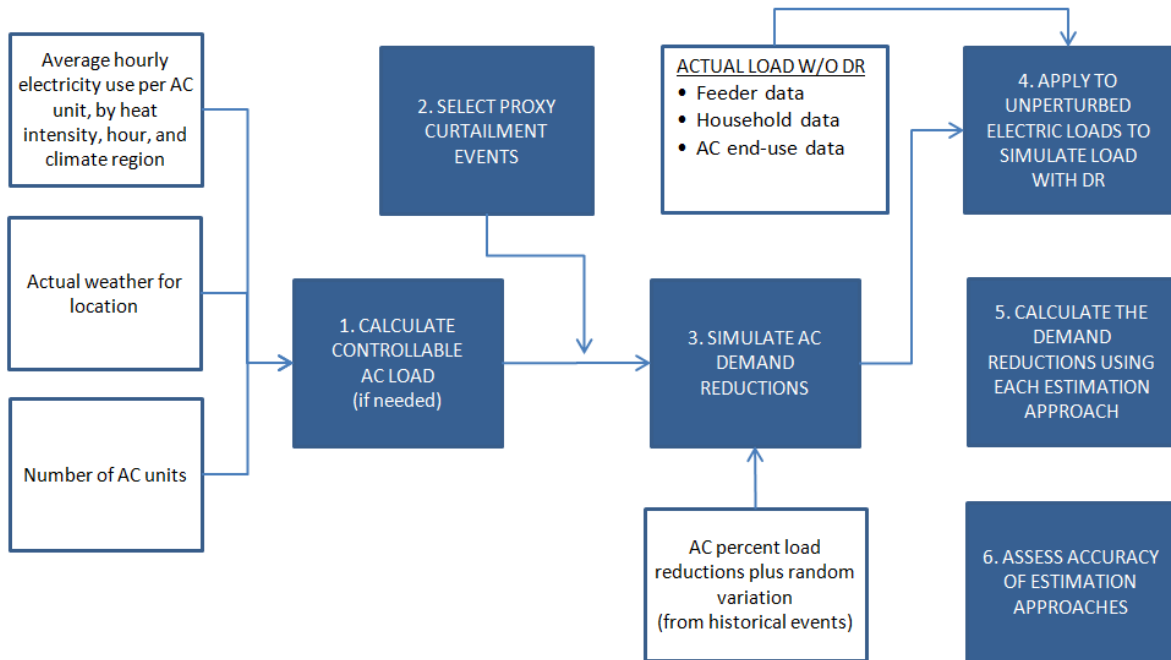
Figure 1: Methodological Framework
