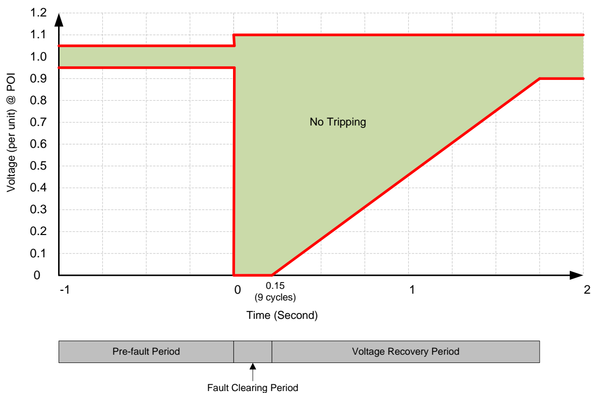
Figure 1: Default Voltage Ride-Through Boundaries For IRRs. The default clearing period is nine cycles or 0.15 seconds. Recovery time to \pm 10\% of per unit voltage should be within 105 cycles, or 1.75 seconds. IRRs should not trip for system voltages within the boundary.
