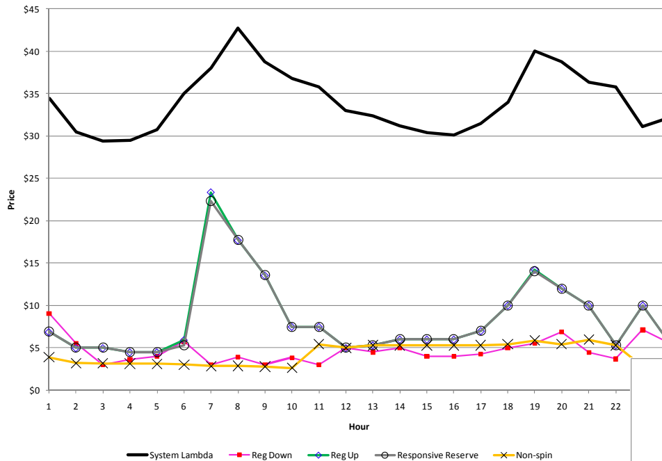
Day-Ahead Electricity And Ancillary Service Prices for 01-Dec-2010
