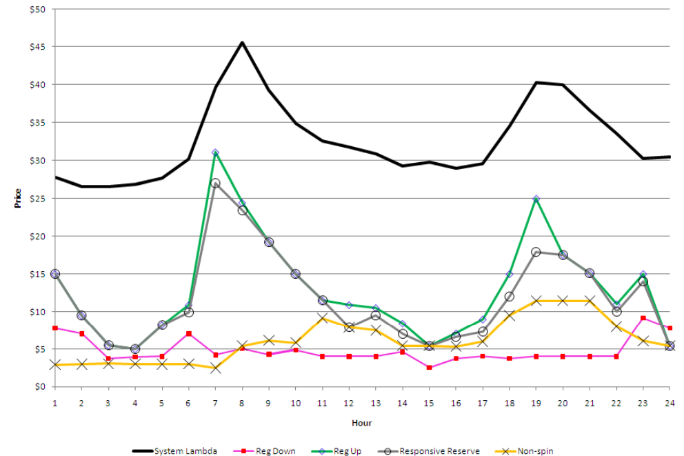
Day-Ahead Electricity And Ancillary Service Prices for 02-Dec-2010
