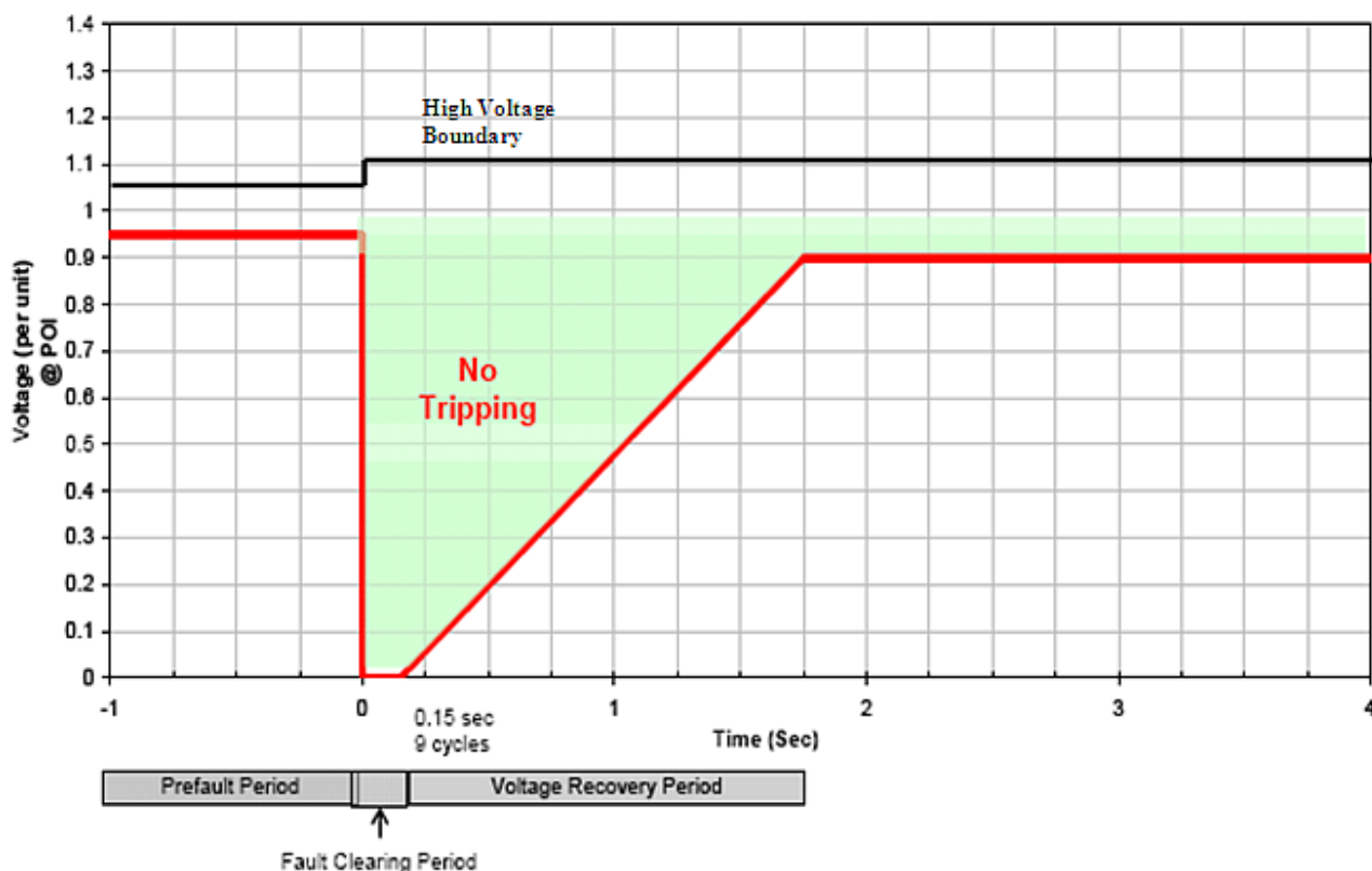
Figure 1: Voltage Ride-Through Boundaries For Wind-powered Generation Resources
