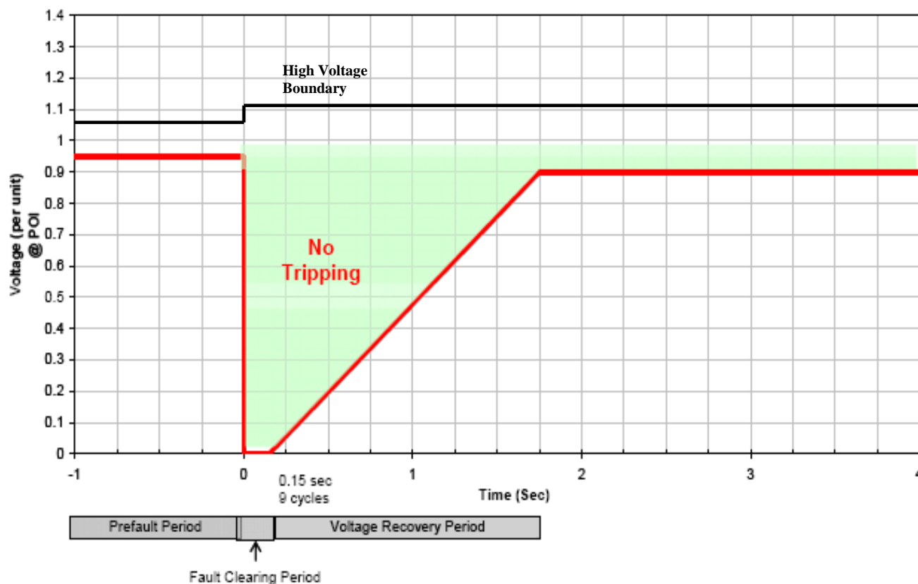
Figure 1: Voltage Ride-Through Boundaries For Wind-powered Generation Resources
