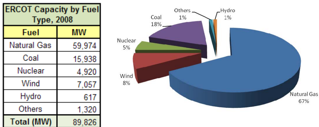
Figure 3-3: ERCOT Generation Capacity by Fuel Type: 2008
