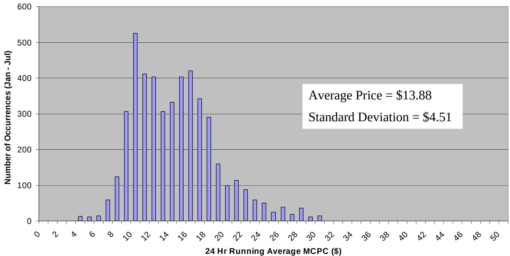
Histogram for Running Average MCPC
