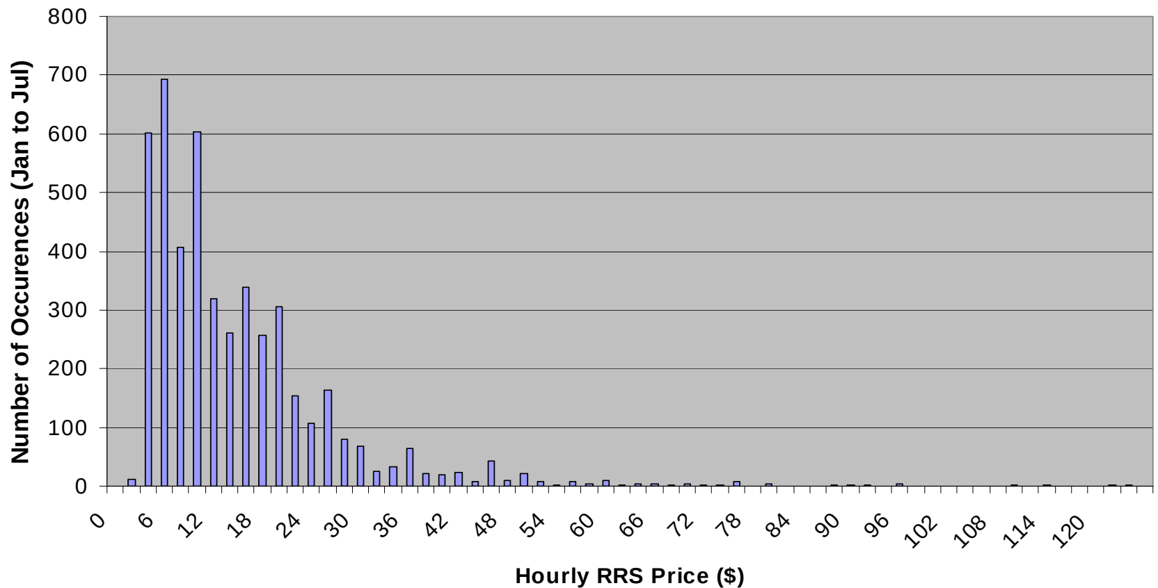
Histogram of Hourly RRS Prices
