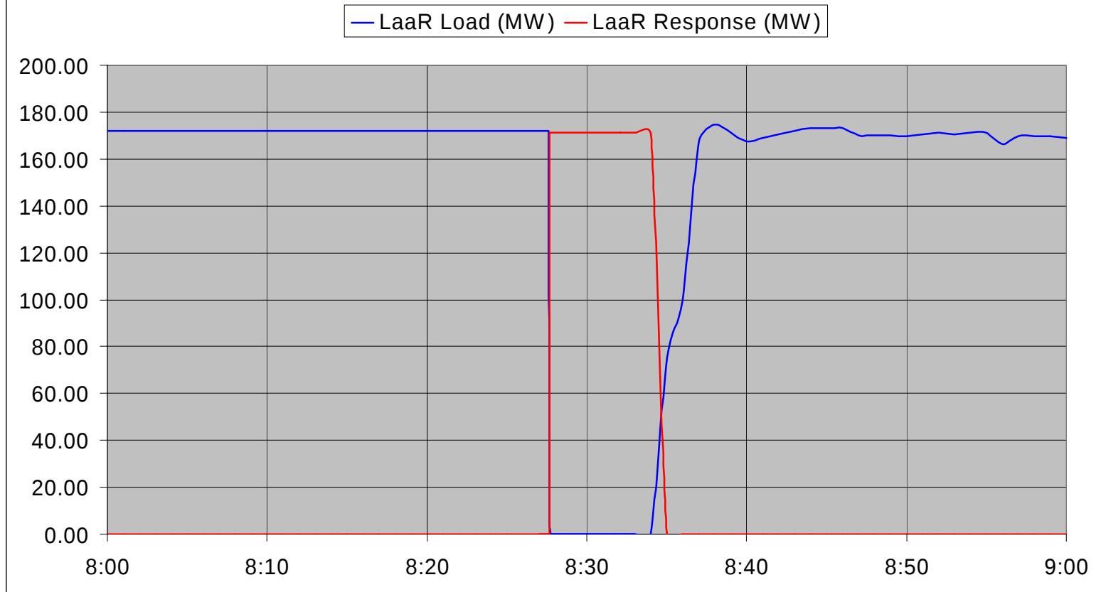
LaaR Response to Under Frequency Event on 12/7/04
