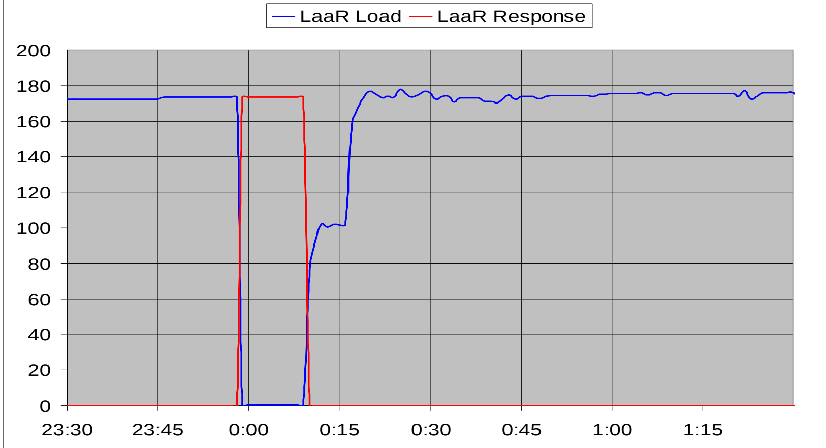
LaaR Response to UF Event on 12/22/04
