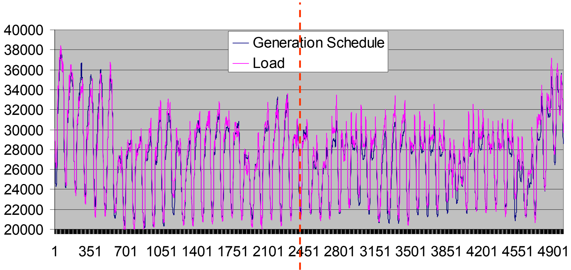
Generation Schedule vs. Load (10/7 -11/27)
