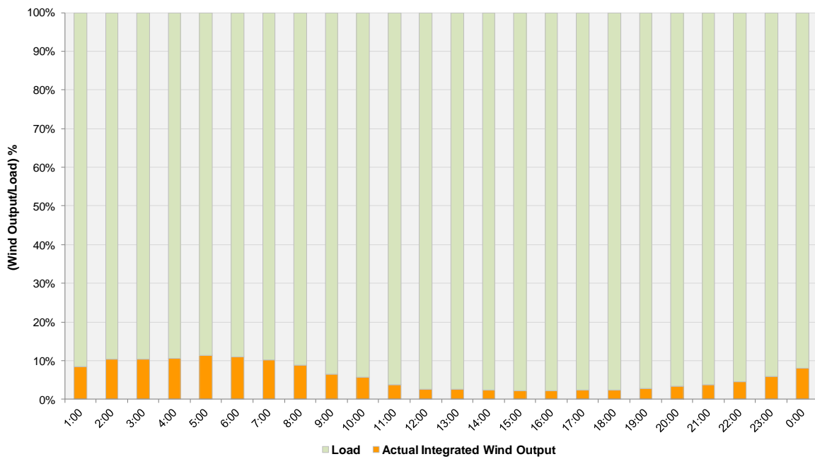
Actual Wind Output as a Percentage of the ERCOT Load 08-05-2011
