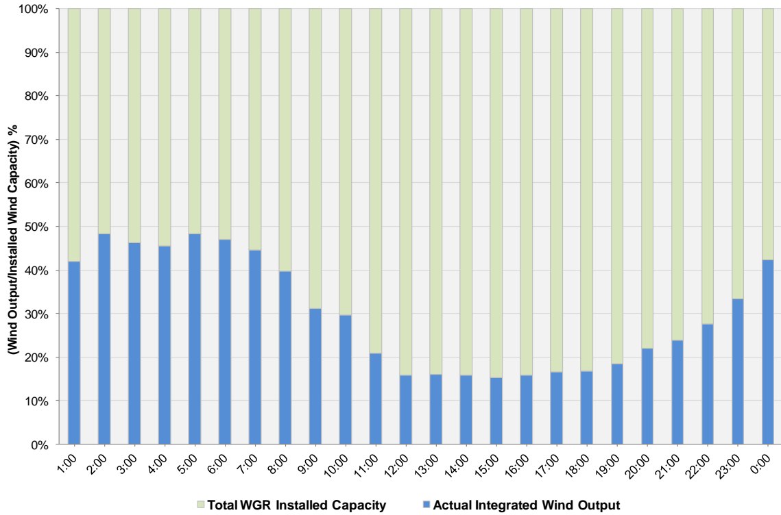
Actual Wind Output as a Percentage of the Total Installed Wind Capacity 08-05-2011
